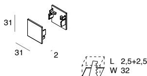
TESTATE TERMINALI (2 pz.) END CAPS (2 pcs)
