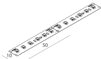
SMD 2835 (120 LED/m) Biadesivo - sezionabile ogni 50mm (6 LED) Biadhesive - cuttable every 50mm (6 LED)
