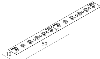
SMD 2835 (120 LED/m) Biadesivo - sezionabile ogni 50mm (6 LED) Biadhesive - cuttable every 50mm (6 LED)
